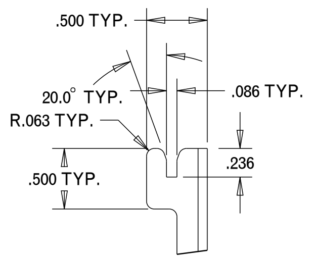
DETAIL A SCALE 1.250 (ALL DIMS THIS VIEW ARE 4X)
